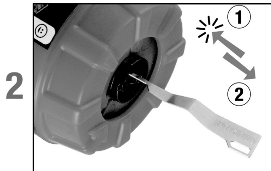
A Insert the SmartKey tool into the small hole (next to the keyway) on the cylinder face, and push with force till it goes all the way in, then remove the SmartKey tool.
