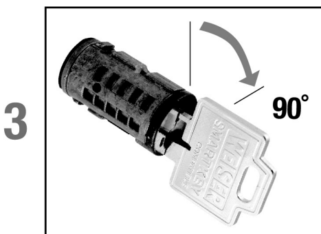
A While holding the cylinder body stationary, rotate the key back to the home position.
